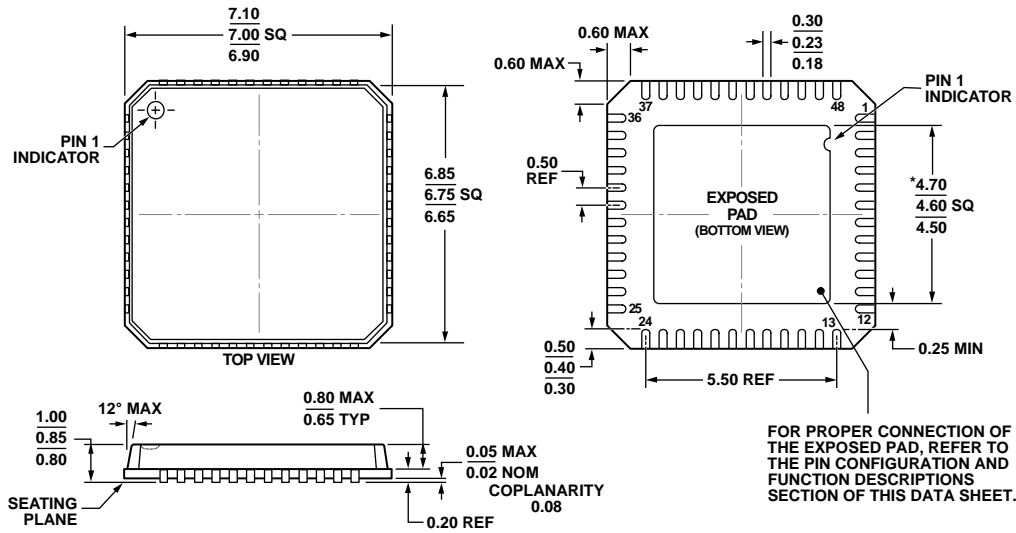
Figure 34. 48-Lead Lead Frame Chip Scale Package [LFCSP_VQ] 7 mm × 7 mm Body, Very Thin Quad (CP-48-12) Dimensions shown in millimeters
