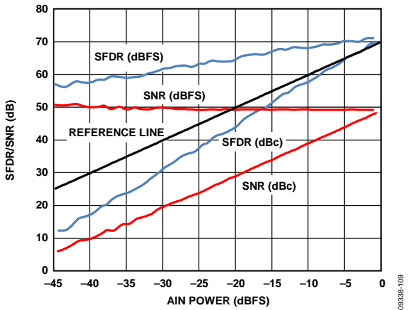
Figure 9. SFDR/SNR vs. Input Amplitude (AIN) with f_{IN} = 2.2 MHz
